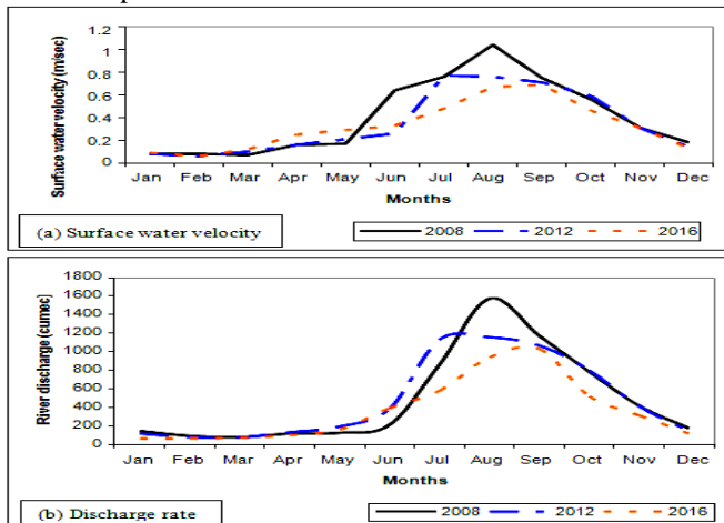
Fig 8. Buriganga River (A) Surface Water Velocity (M/Sec) and (B) Discharge Rate (Cumec) Measured at Millbarak during 2008, 2012 and 2016
